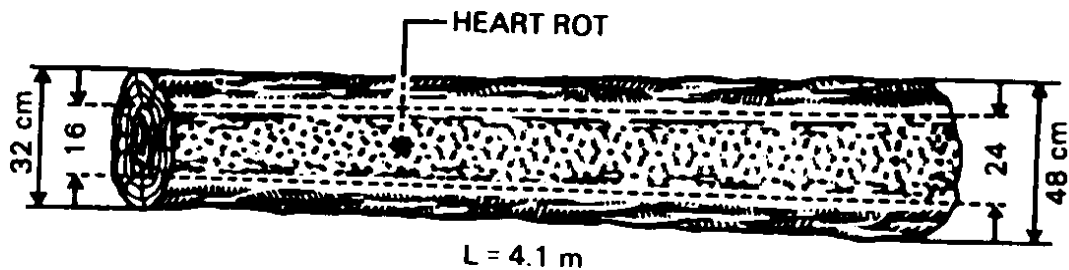
Figure 18 Full length heart rot (showing at both ends)
