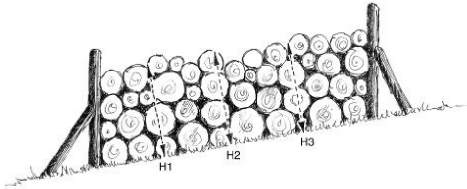
Figure 13 Measuring height of stack piled on a slope
