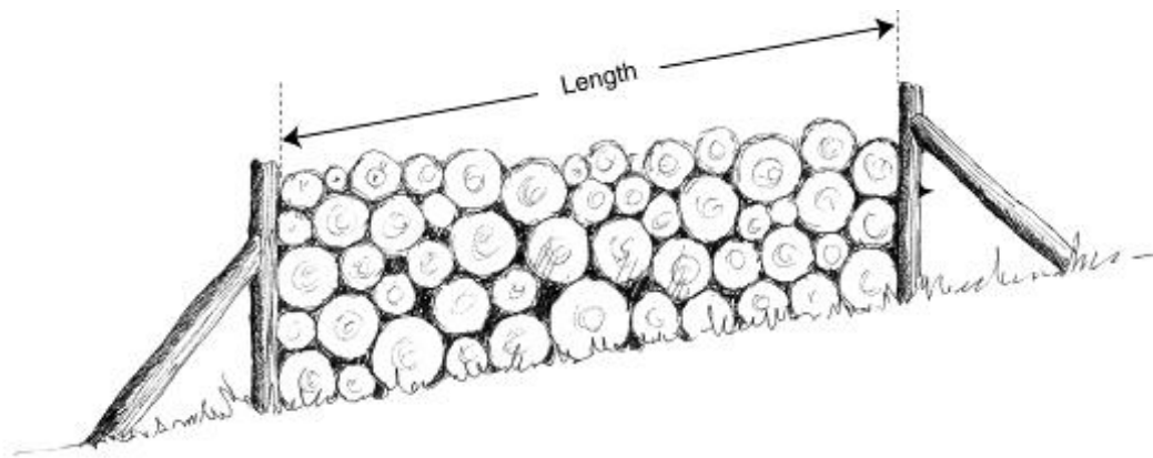
Figure 9 Measuring length of stack on a slope
