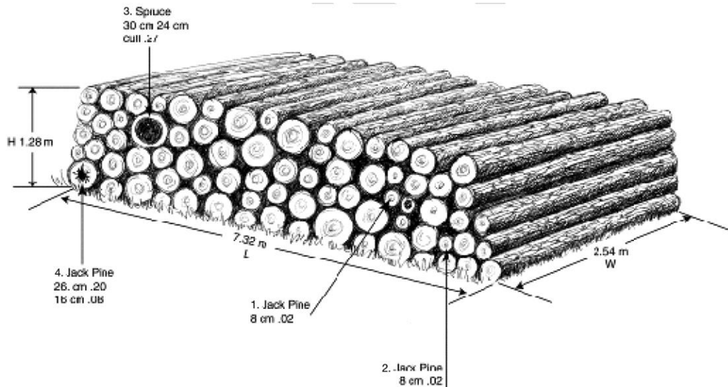
Figure 29 Net pile volume
