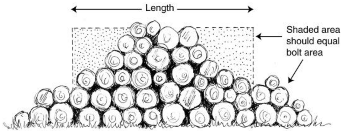
Figure 8 Measuring length of stack when stack drops off at both ends
