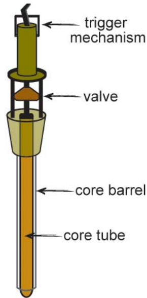
Figure 10. Kajak-Brinkhurst core sampler (British Columbia MWLAP (2003))
