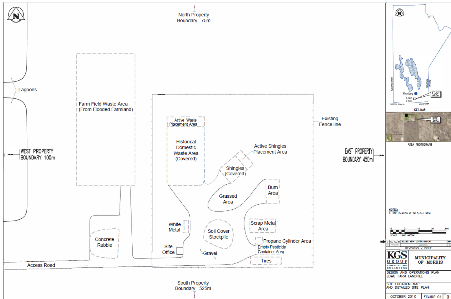
Figure 1 Facility Layout
