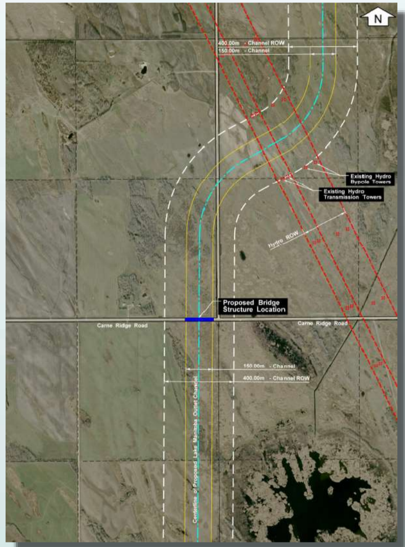
Carne Ridge Road Bridge Structure
