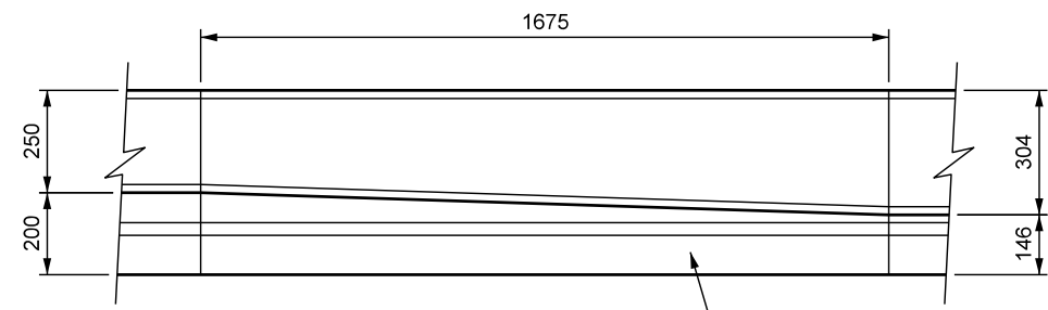
PLAN SCALE 1:20
