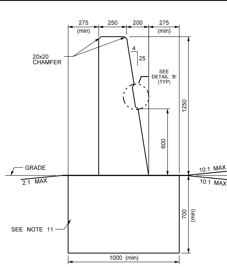
SECTION 'C-C' END SECTION SCALE 1:20
