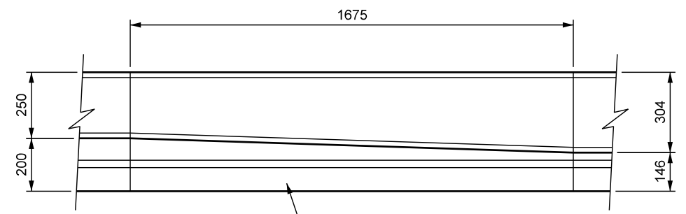
PLAN SCALE 1:20
