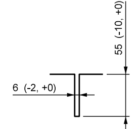
SLIP FORMED BARRIER (SAW CUT) SCALE 1:5
