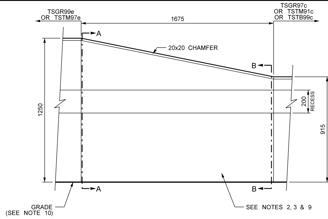
ELEVATION SCALE 1:20
