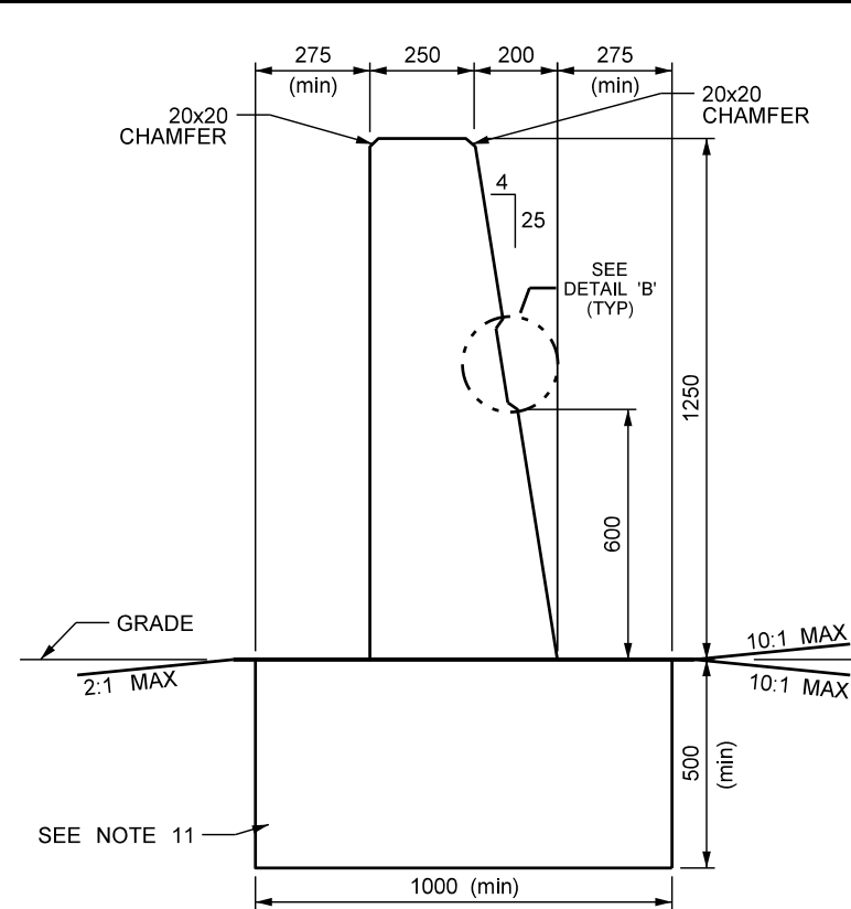
SECTION 'A-A' INTERIOR SECTION SCALE 1:20
