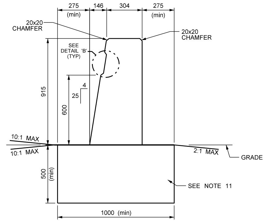
SECTION 'B-B' INTERIOR SECTION SCALE 1:20
