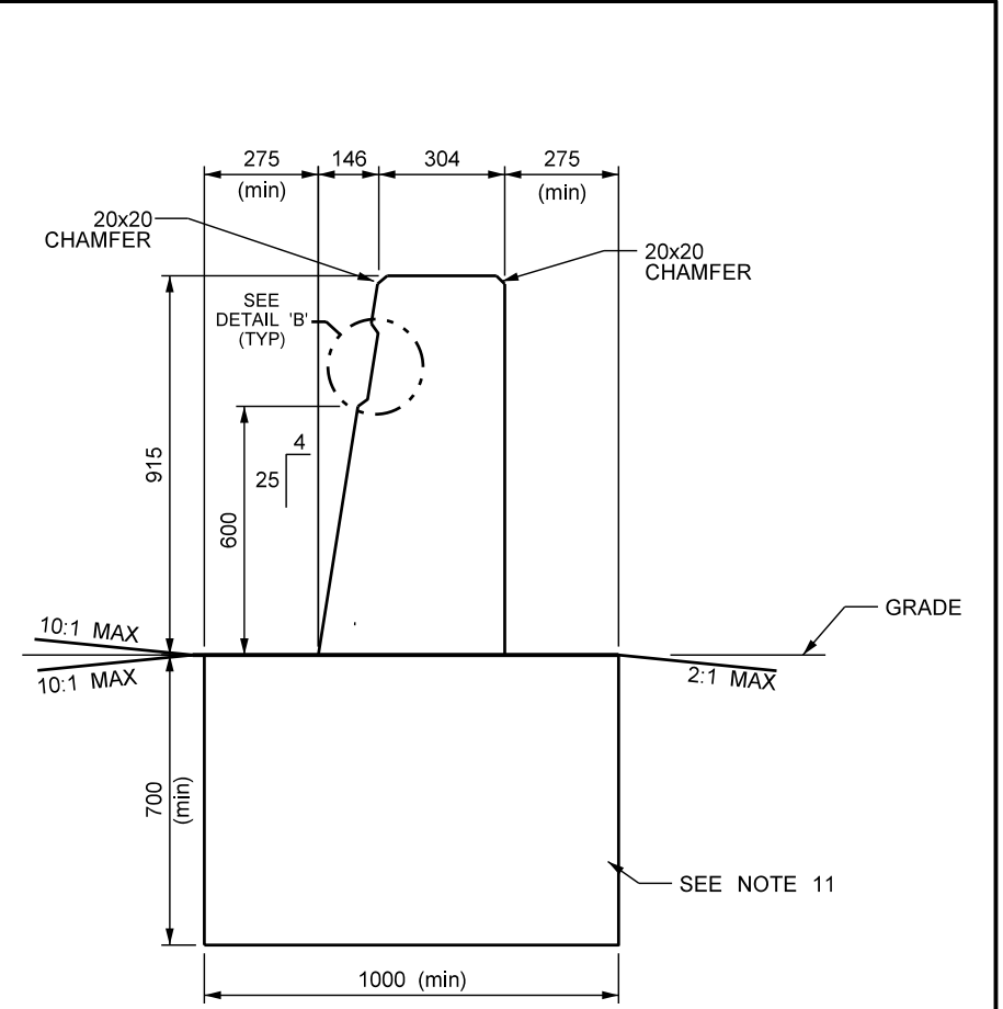
SECTION 'D-D' END SECTION SCALE 1:20
