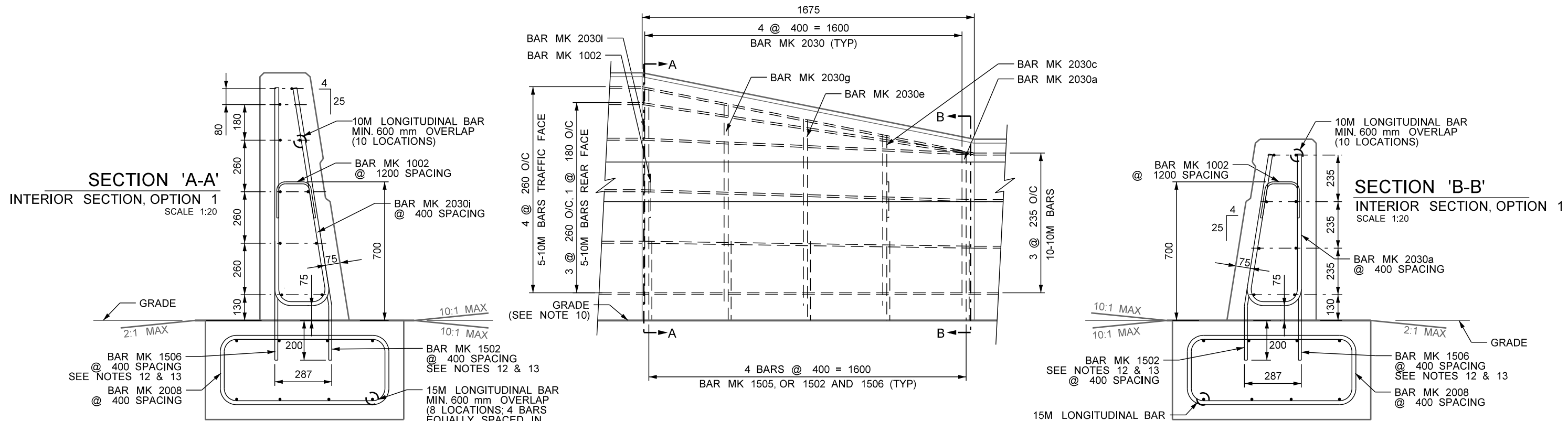
ELEVATION SCALE 1:20
