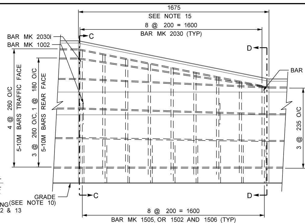
ELEVATION SCALE 1:20
