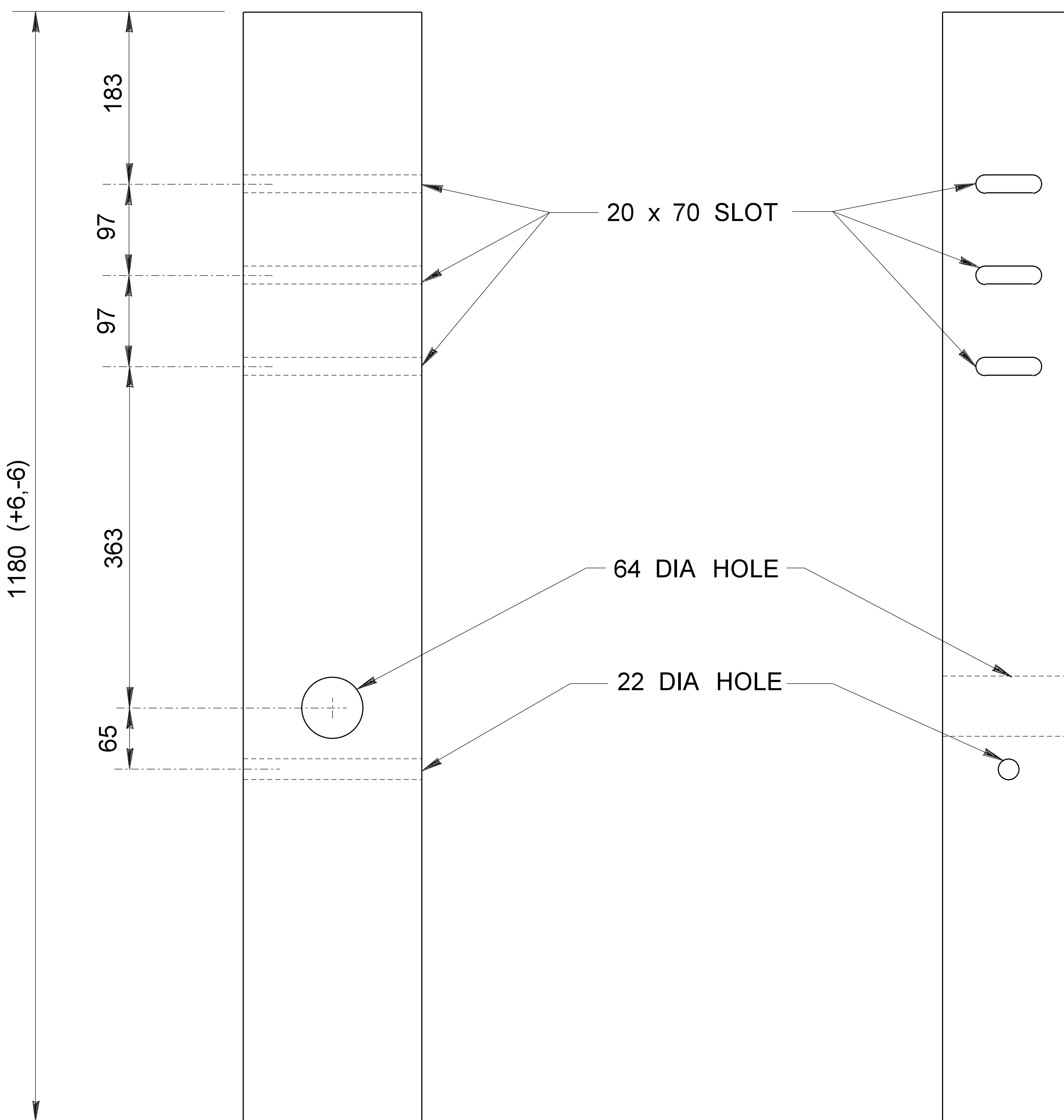
SIDE 1:10
