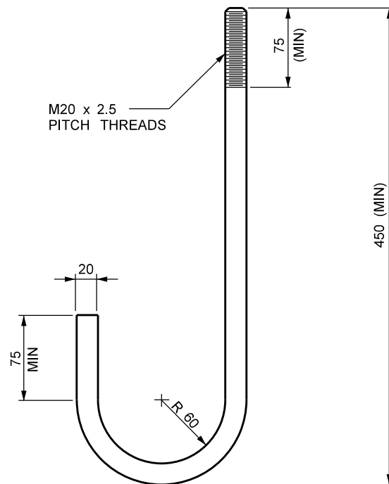
ELEVATION VIEW 1:5
