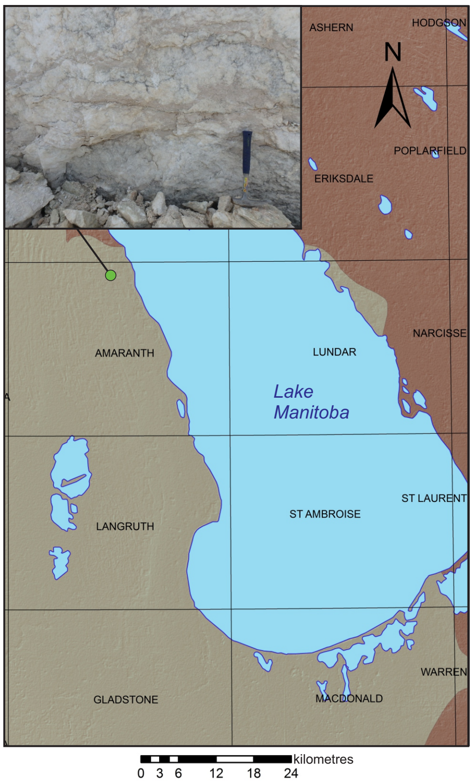
Digital elevation map showing the distribution of the Upper Amaranth Member in green; NTS 50K sheets are labelled. Inlay is of gypsum from an active quarry.
